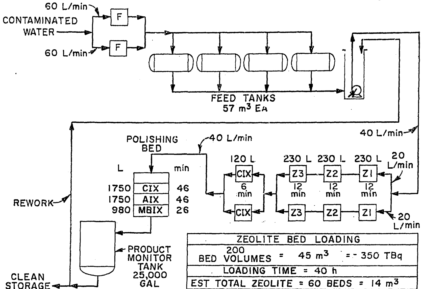
FIG. 5. SDS FLOWSHEET.
