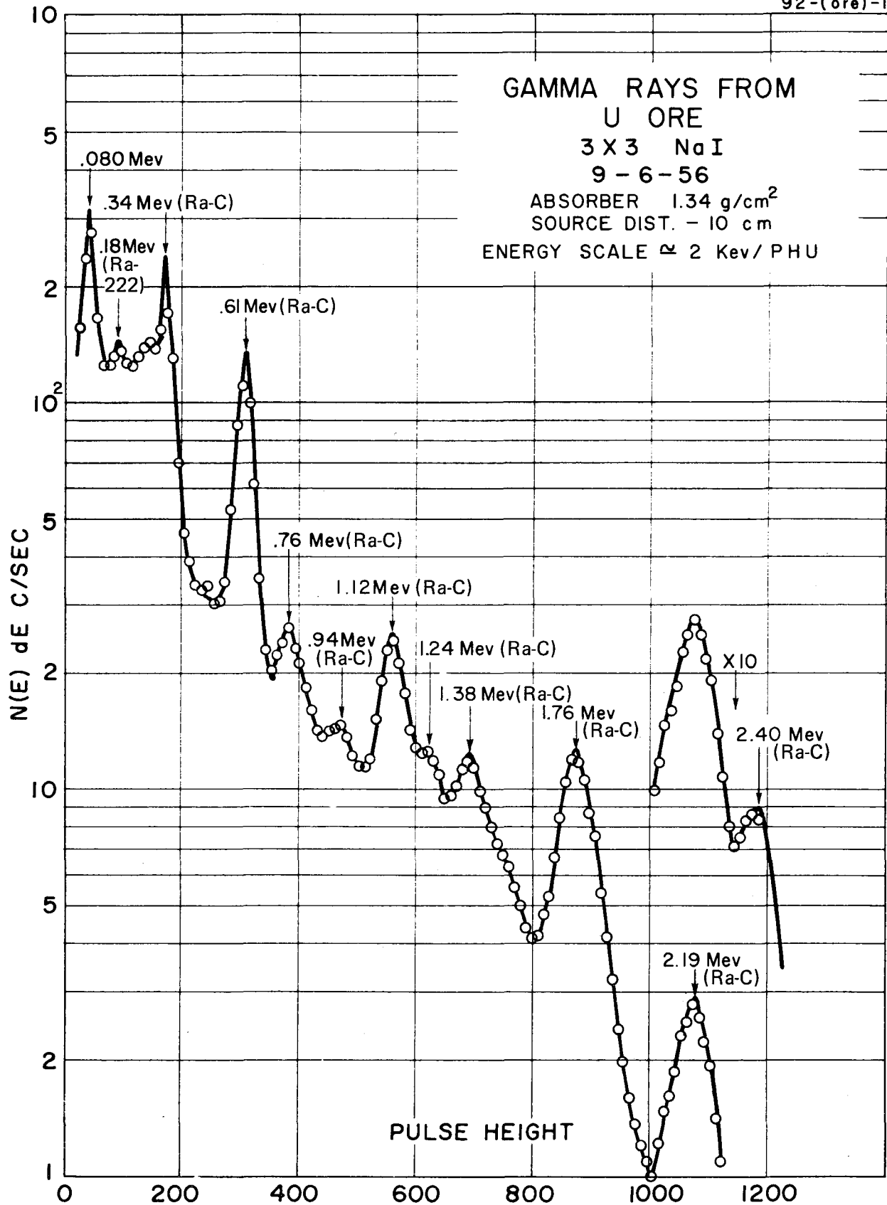
FIGURE 1. PRINCIPAL GAMMA RAYS FROM SHORT-LIVED RADON-222 PROGENY (REF. 1)
