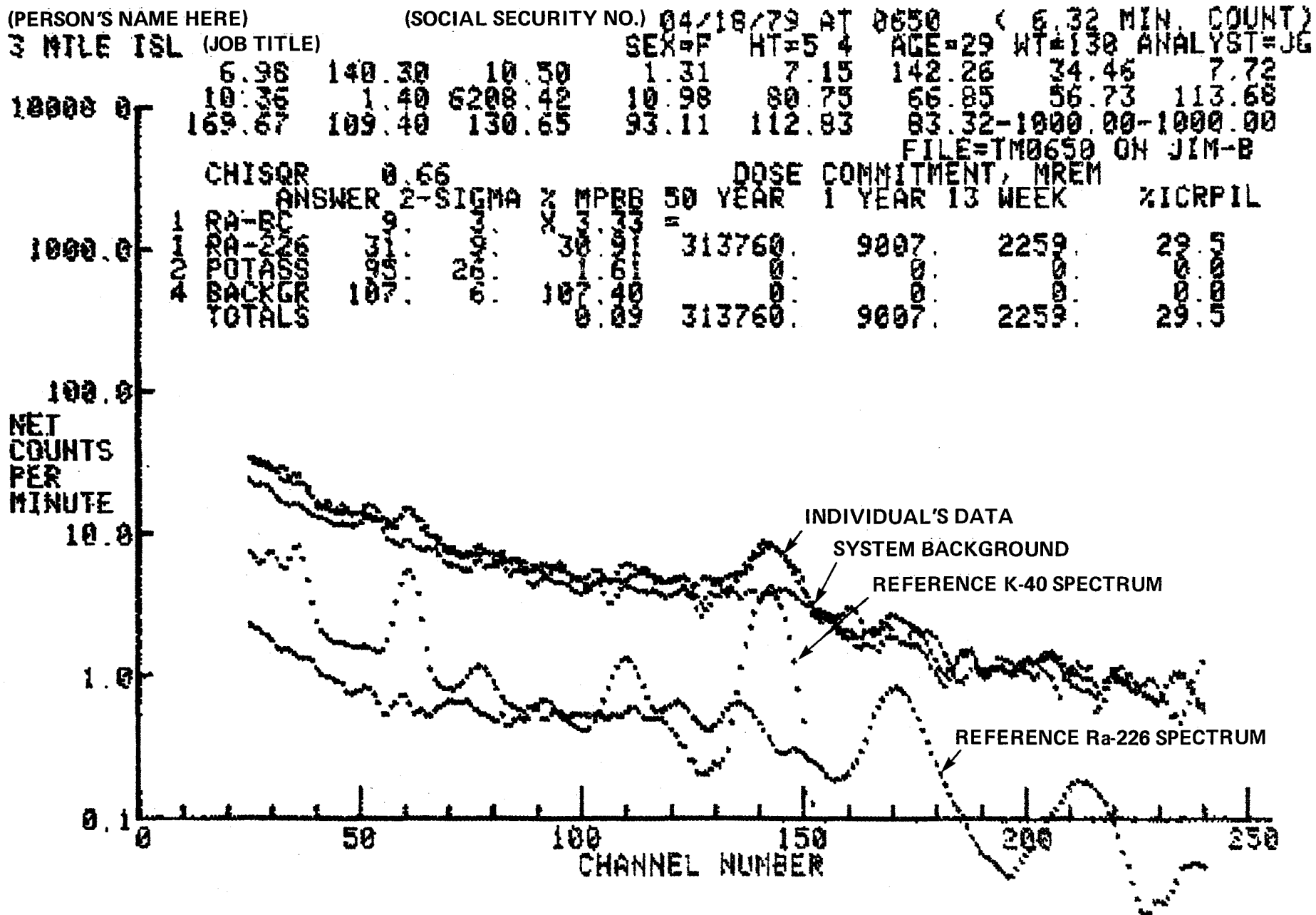
FIGURE 4. EXAMPLE OF GAMMA SPECTRUM AND RESULTS
