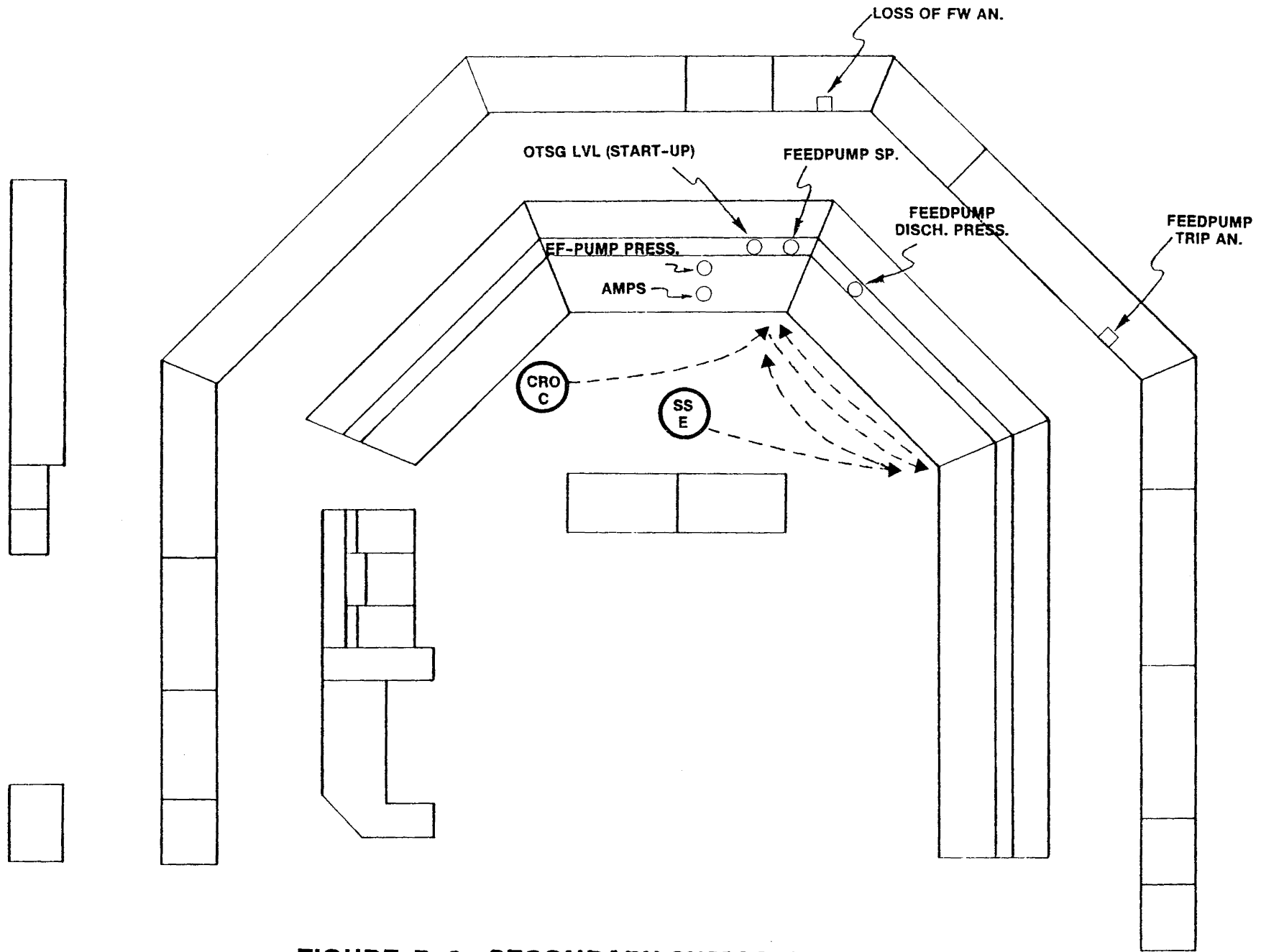
FIGURE B-6 SECONDARY SYSTEM IMMEDIATE ACTIONS
