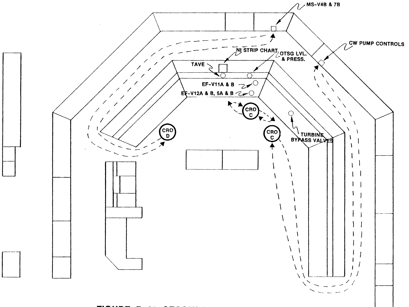
FIGURE B-10 SECONDARY SYSTEM CONTROL (20-150 MINUTES)
